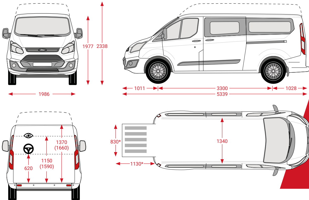
Dimension based on Ford Tourneo Custom with wheelbase L2
